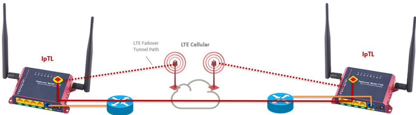
Typical Connection of Two IpTL Appliances
